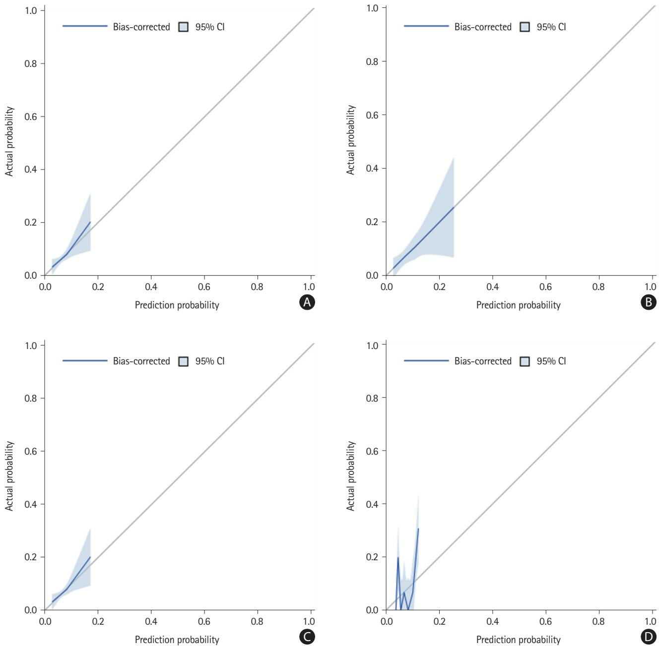
Supplementary Figure 3. Calibration plot of the (A) TAG score, (B) ASIAN score, (C) IER-SICH nomogram, and (D) STBA score using Hosmer–Lemeshow test. TAG, TICI-ASPECTS-glucose; ASIAN, ASPECTS, baseline glucose, poor collateral circulation, passes with retriever, and onset-to-groin puncture time; IER-SICH, Italian Registry of Endovascular Stroke Treatment in Acute Stroke–symptomatic intracerebral hemorrhage; STBA, systolic blood pressure, time from acute ischemic stroke until groin puncture, blood glucose, and ASPECTS; CI, confidence interval.
